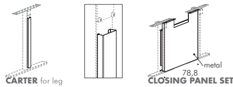
CARTER for leg PT9201 L5 P2,6 H56 CLOSING PANEL SET PT9202 x1
